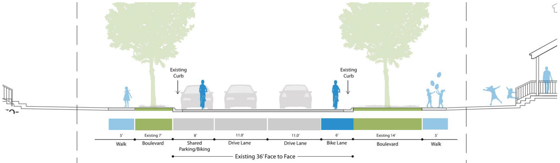
Existing Street Configuration to Remain
